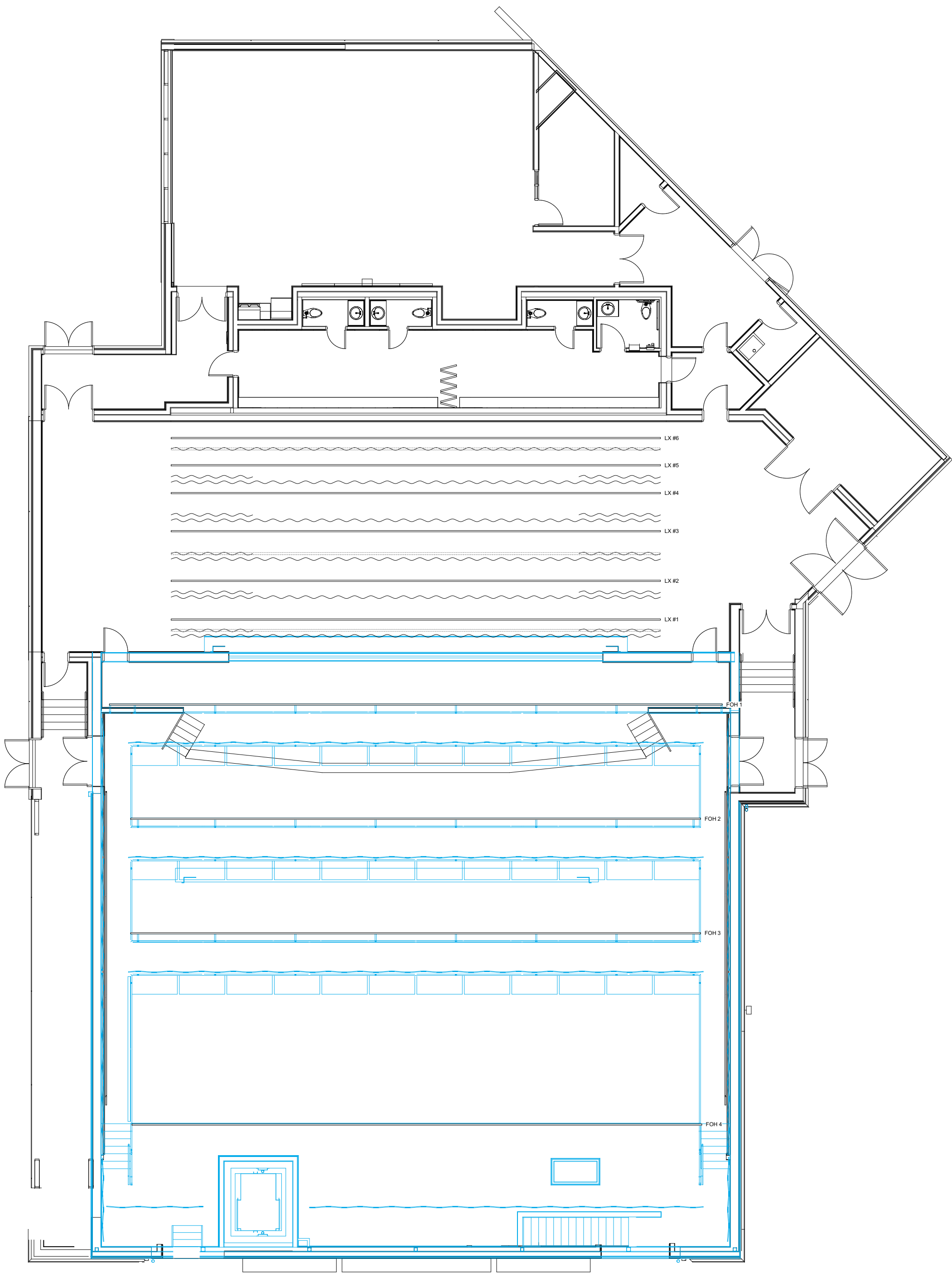
1 Full Plan View - Catwalk Scale: 3/32" = 1'-0"
