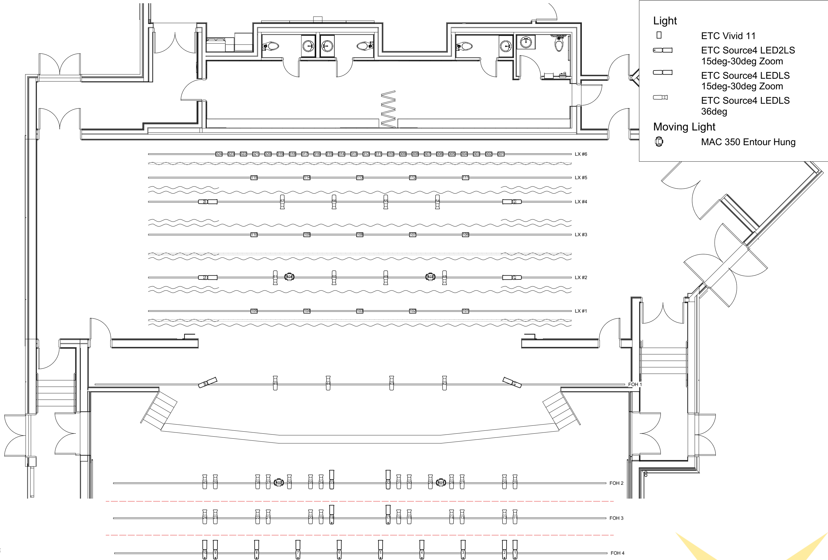
1 Lighting Plot Scale: 1/8" = 1'-0"
