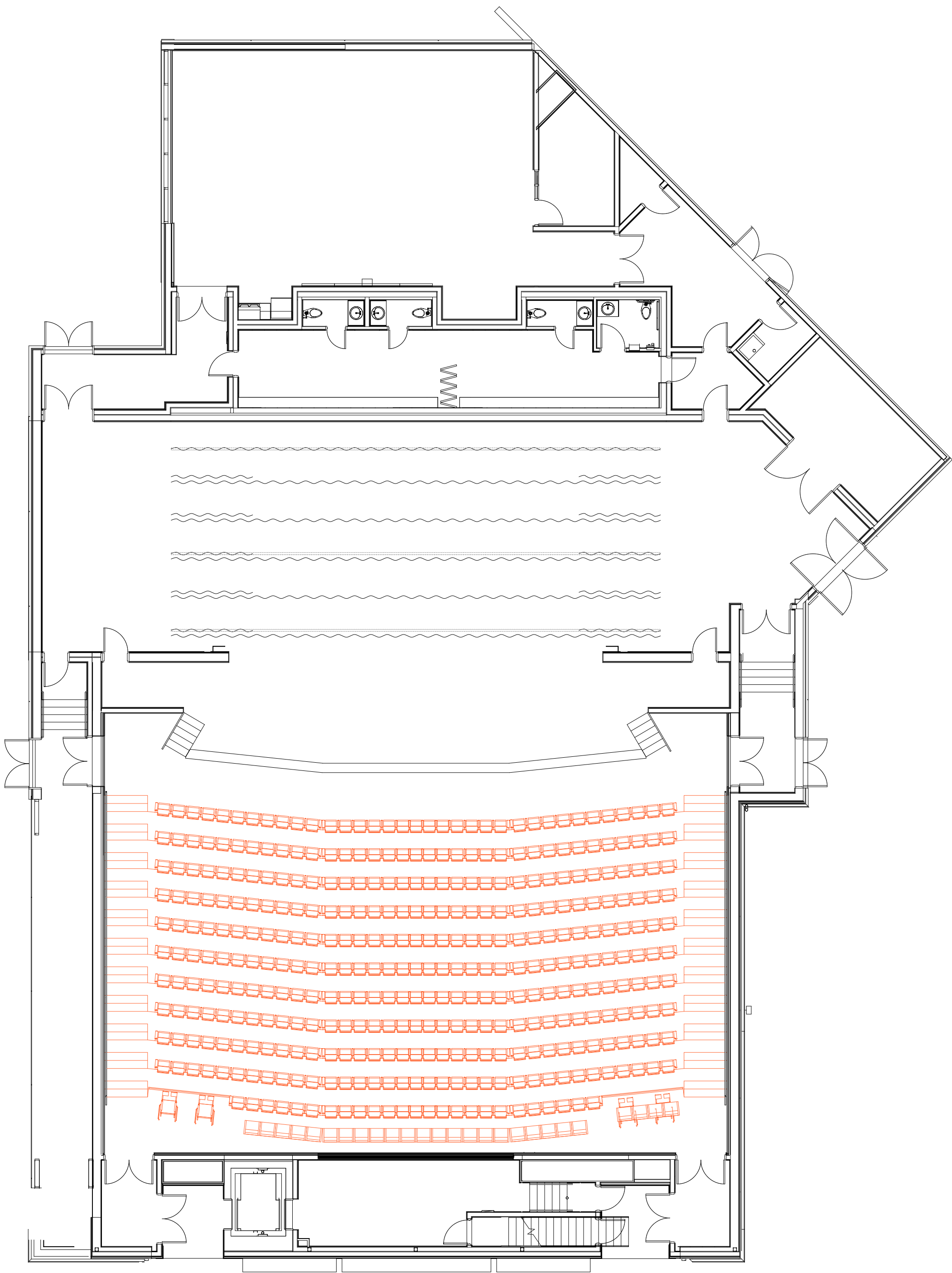
1 Full Plan View Scale: 3/32" = 1'-0"
